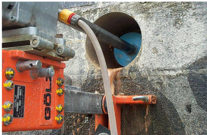
Core Drilling
