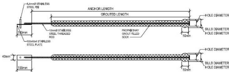
ANCHOR TYPE C3 - UPPER WATERSHED ANCHORS WHERE STONES REMAIN IN PLACE
