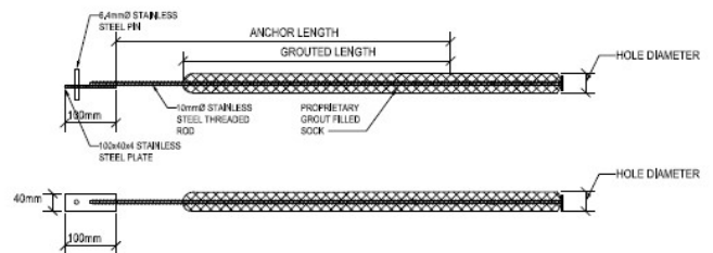
ANCHOR TYPE C6 - LOWER WATERSHED ANCHORS WHERE STONES ARE REMOVED
