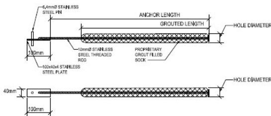
ANCHOR TYPE C3 - UPPER WATERSHED ANCHORS WHERE STONES REMAIN IN PLACE
