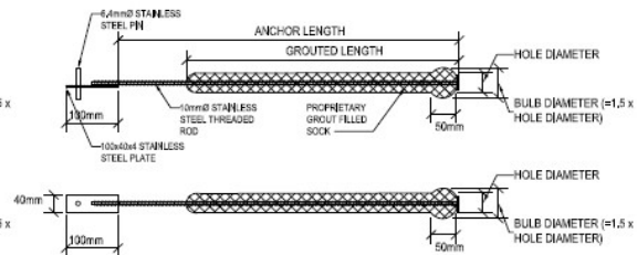
ANCHOR TYPE C6 - LOWER WATERSHED ANCHORS WHERE STONES ARE REMOVED
