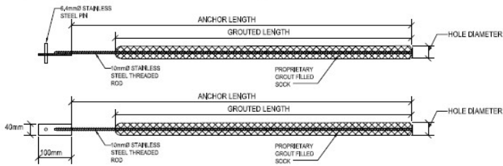
ANCHOR TYPE C2 - LOWER WATERSHED AND WINDOW HEAD COMBINATION ANCHORS
