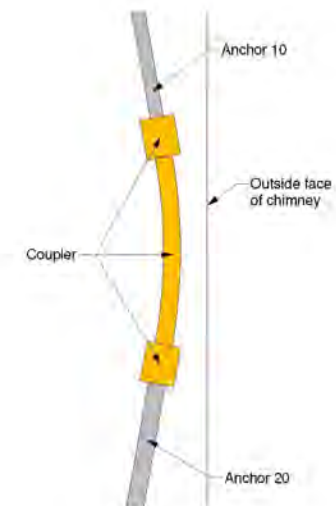
DETAIL 1 SECTION THROUGH ANCHOR 20 & 10 COUPLER (1:10)
