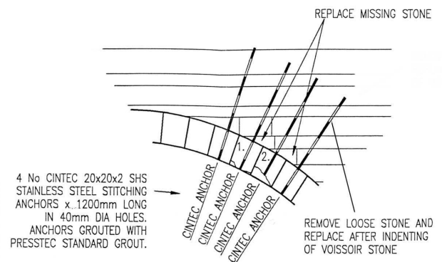
PART ELEVATION OF VOISSOIRS/SPANDREL FACE.
